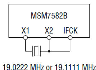
Figure 2 How to Use IFCK, X1, and X2
