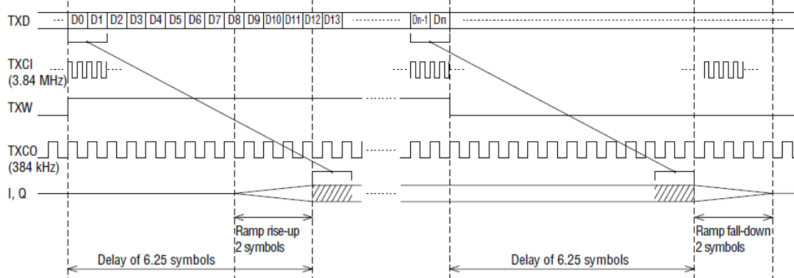
Figure 1 Transmit Timing Diagram
