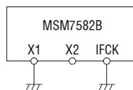
Figure 2 How to Use IFCK, X1, and X2
