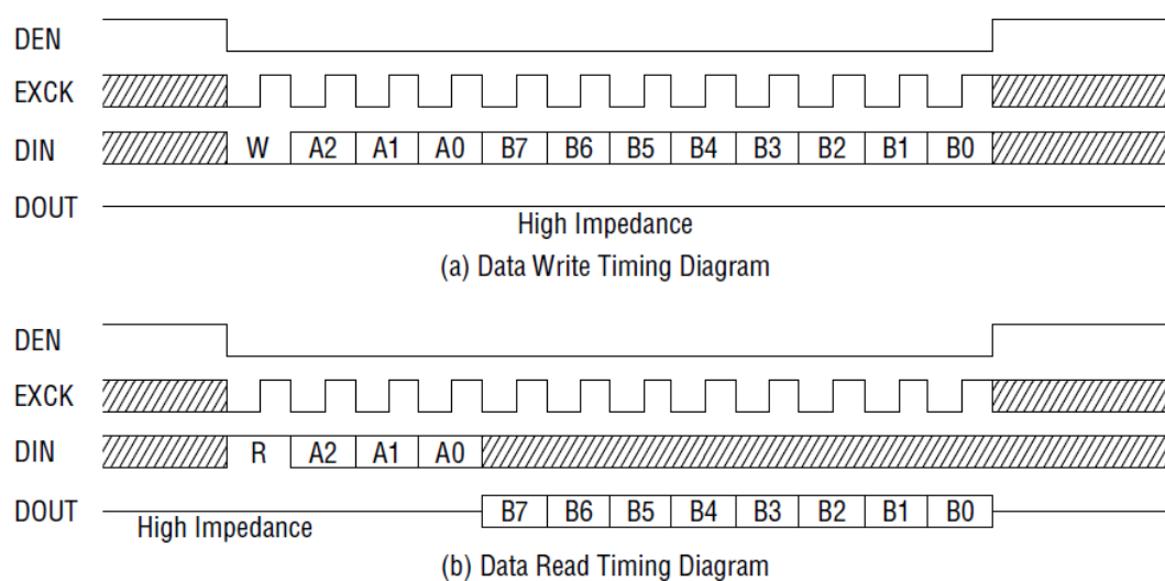
Figure 5 MCU Interface Input/Output Timing Diagram
