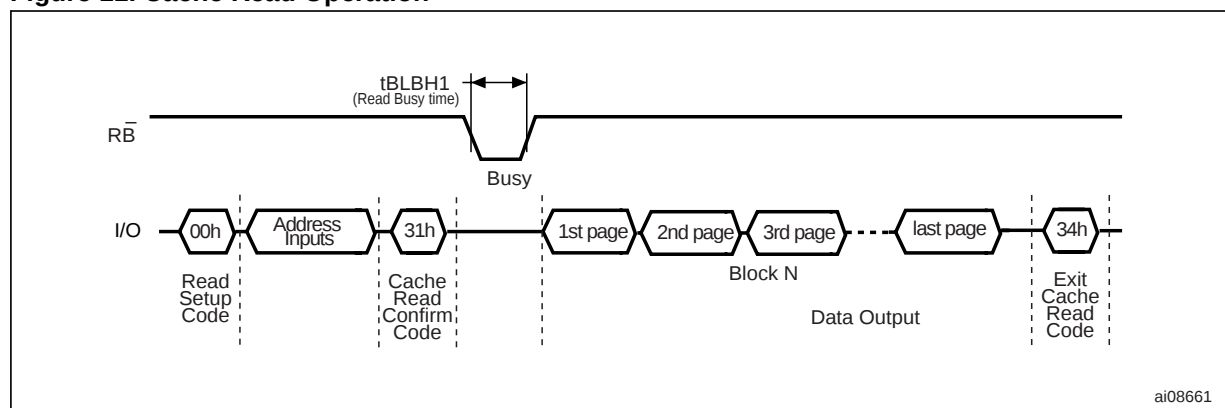
Figure 11. Cache Read Operation
