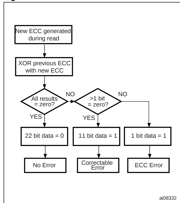
Figure 24. Error Detection
