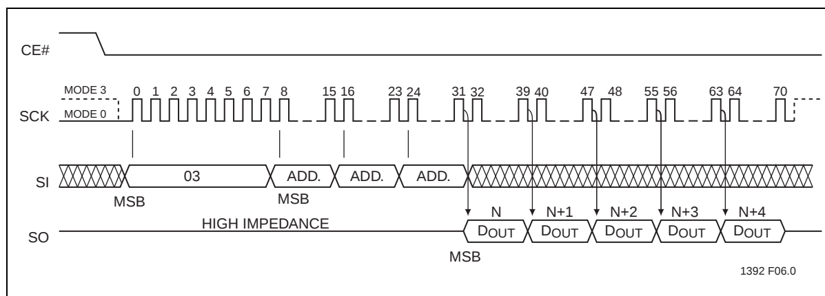
Figure 6: Read Sequence
