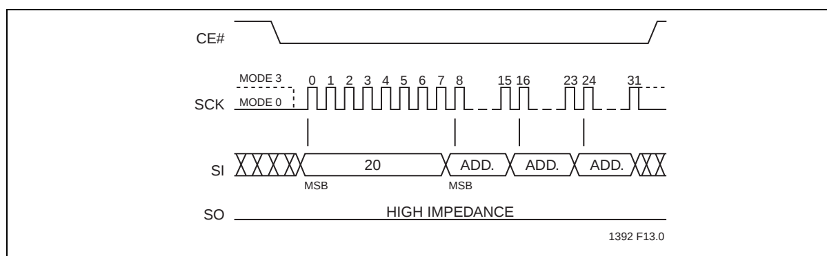
Figure 12: Sector-Erase Sequence
