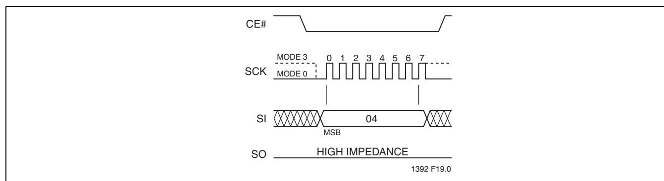
FIGURE 18: Write Disable (WRDI) Sequence
