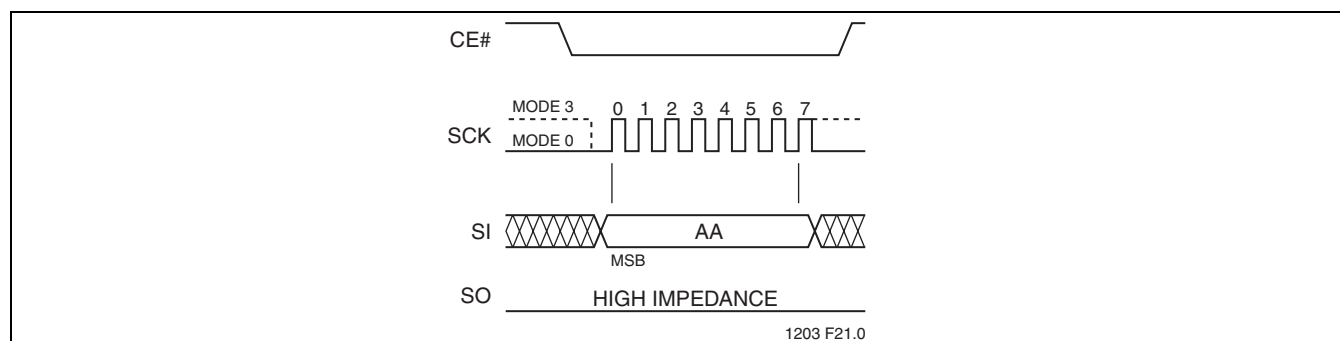
FIGURE 20: Enable-Hold Sequence
