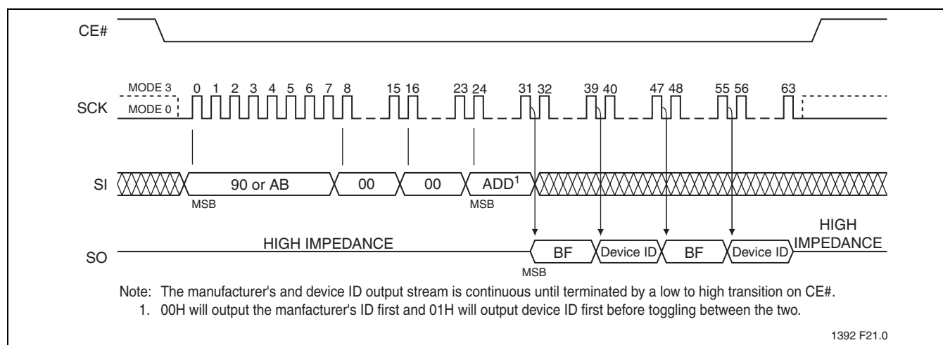
FIGURE 21: Read-ID Sequence
