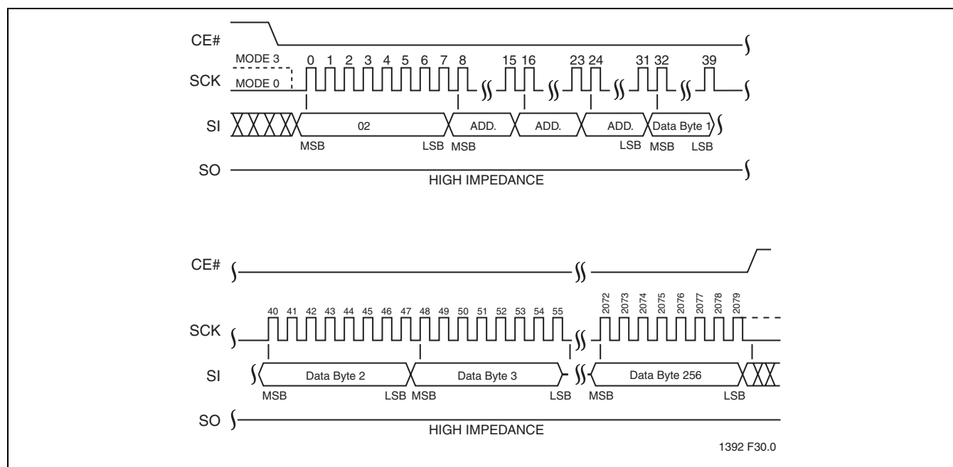
FIGURE 10: Page-Program Sequence
