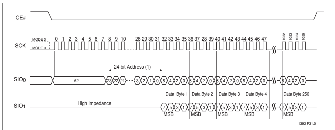
FIGURE 11: Dual-Input Page-Program
