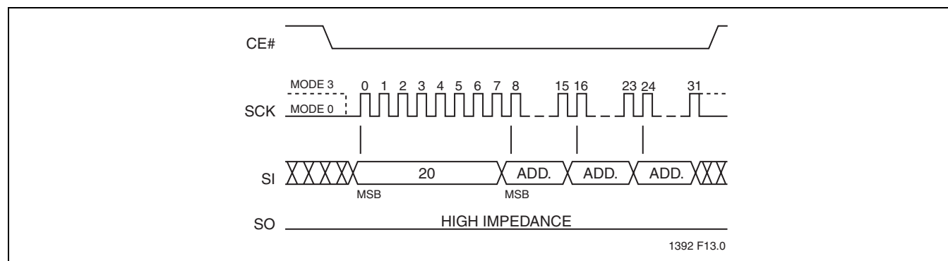
FIGURE 12: Sector-Erase Sequence
