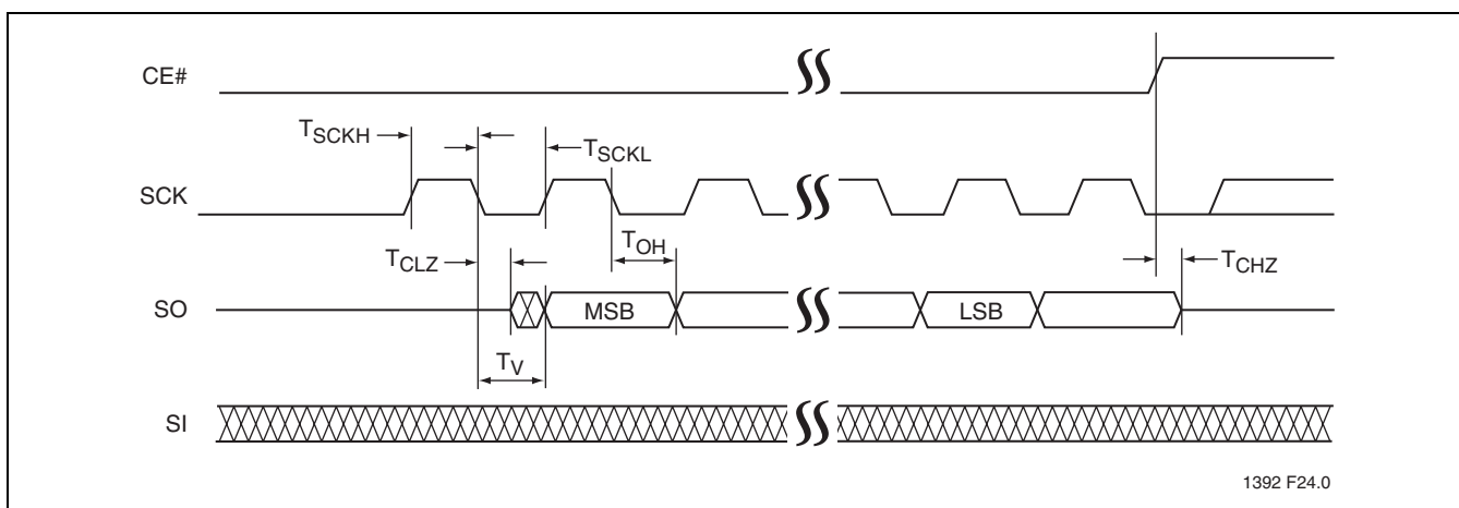
FIGURE 24: Serial Output Timing Diagram
