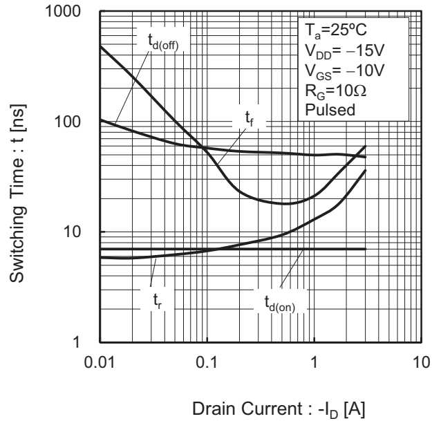
Fig.19 Switching Characteristics
