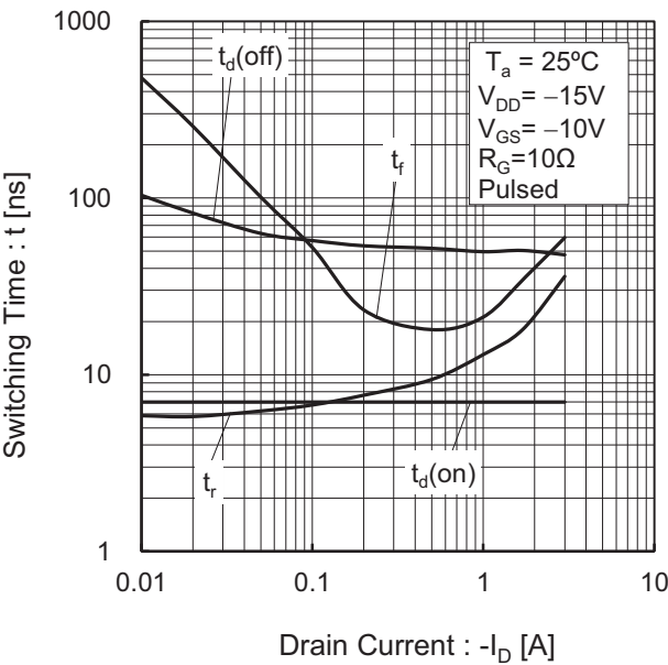
Fig.19 Switching Characteristics
