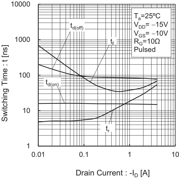
Fig.19 Switching Characteristics
