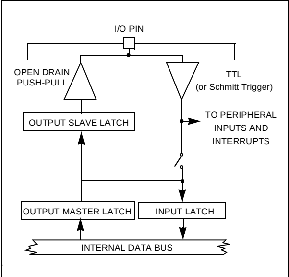
Figure 39. Output Configuration
