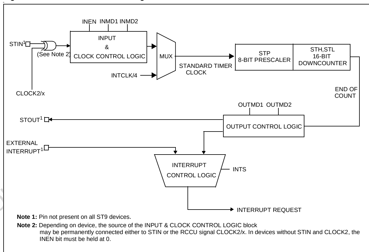
Figure 46. Standard Timer Block Diagram
