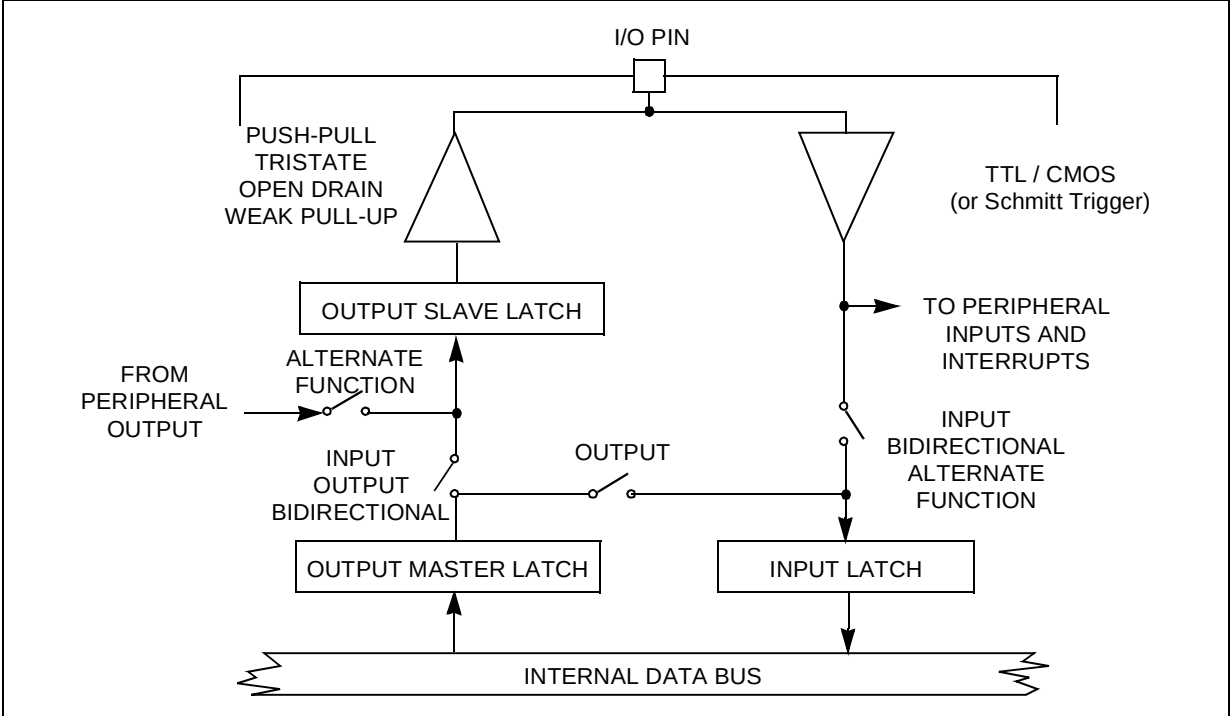
Figure 38. Input Configuration
