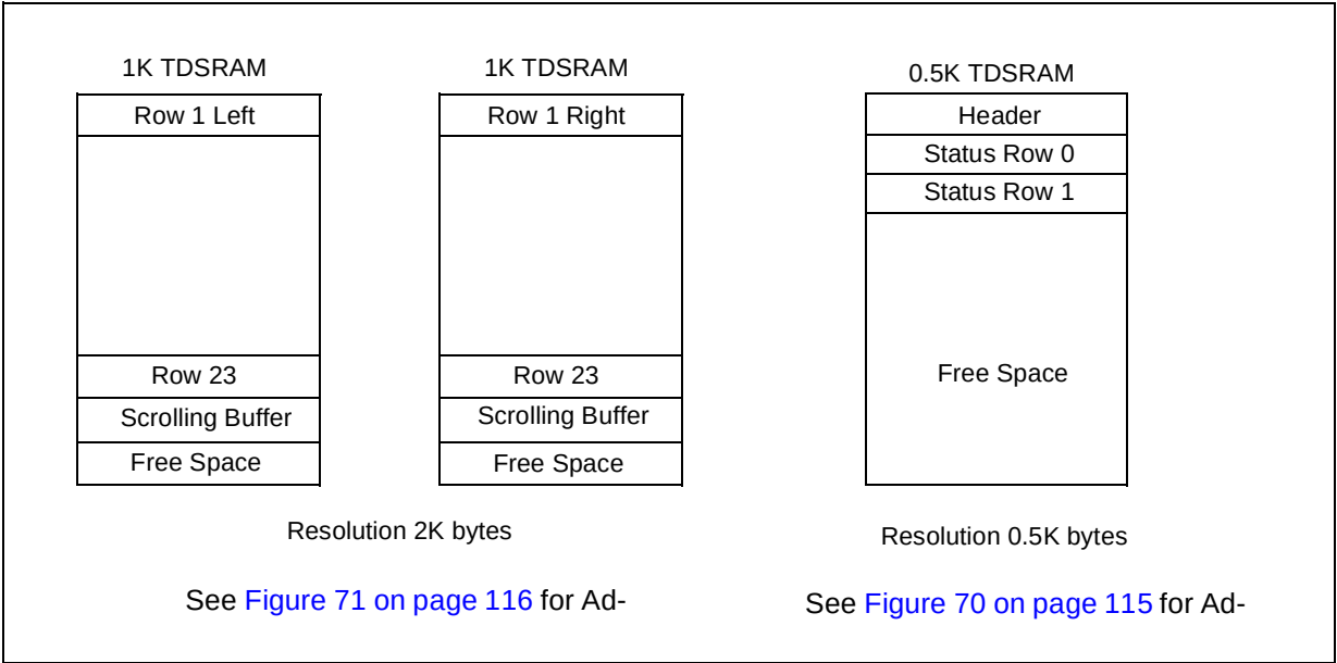
Figure 75. Serial Mode (80 Characters) - Page Mapping
