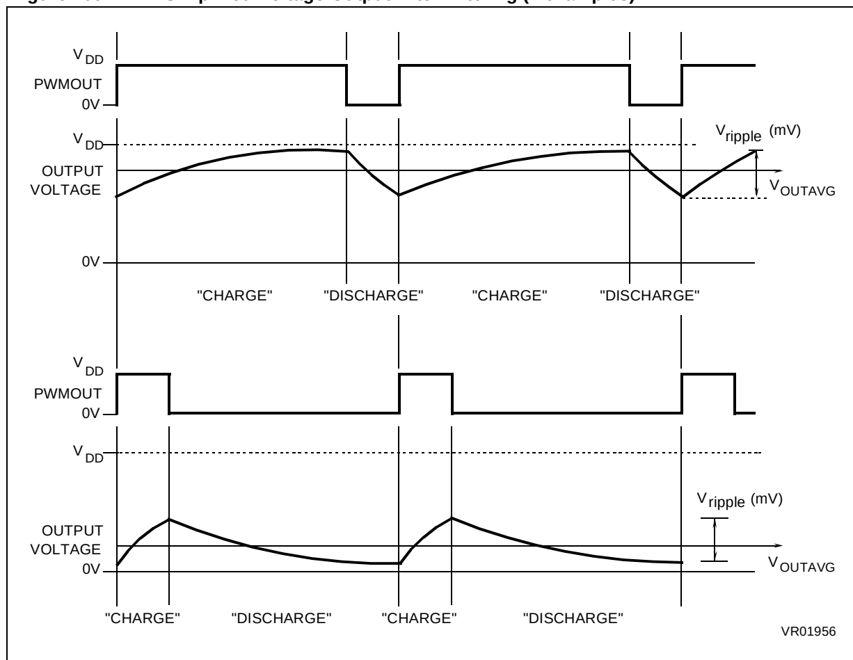
Figure 109. PWM Simplified Voltage Output After Filtering (2 examples)
