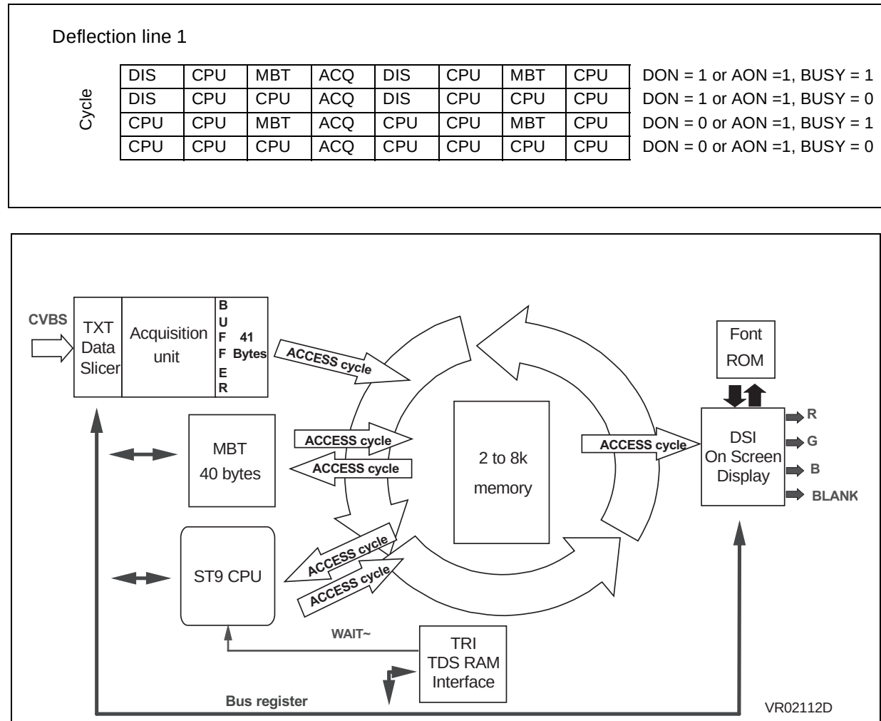
Figure 48. Timesharing Slot Configurations
