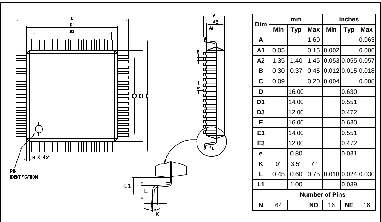
Figure 115. 64-Pin Thin Quad Flat Package
