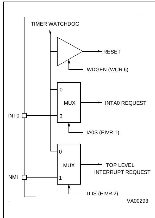
Figure 45. Interrupt Sources
