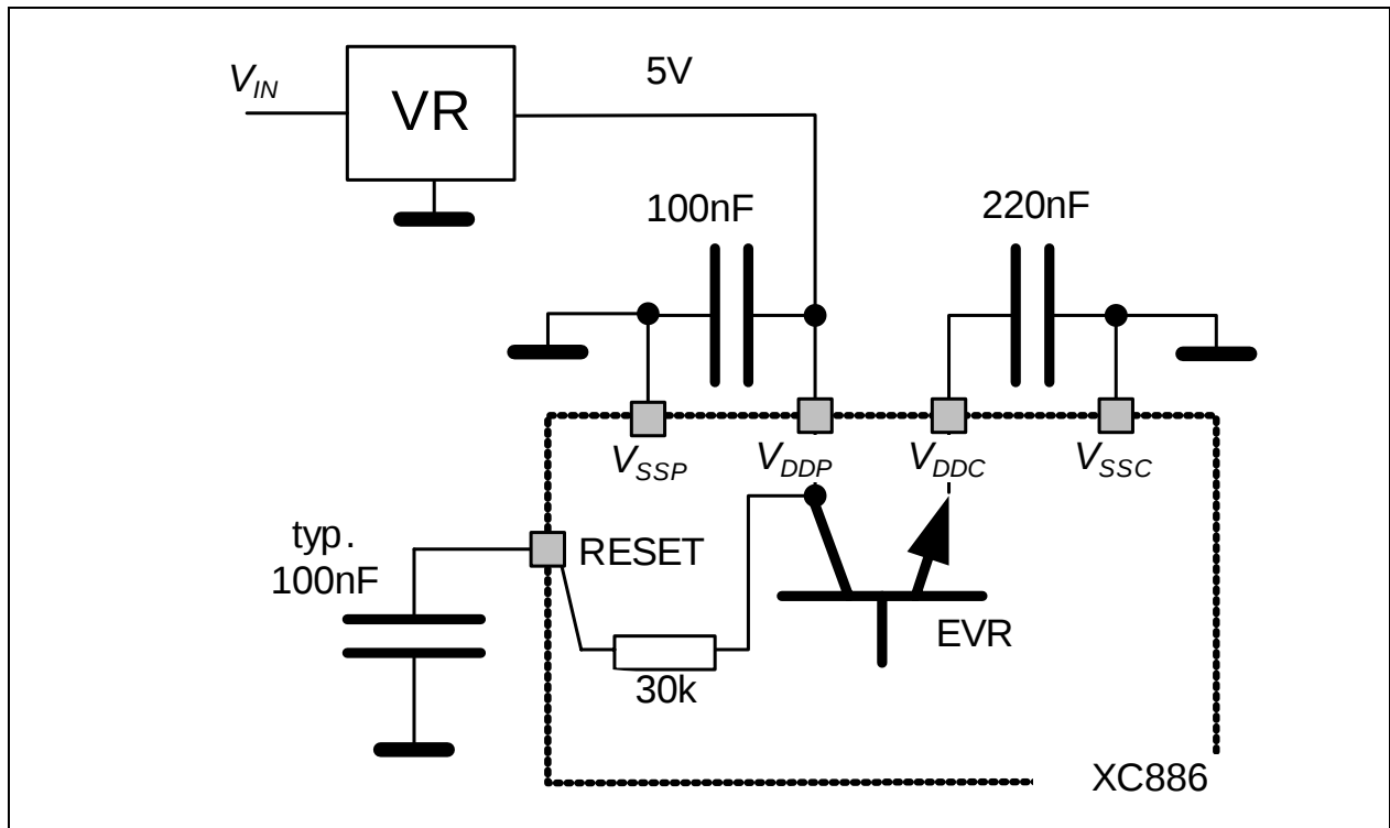
Figure 21 Reset Circuitry
