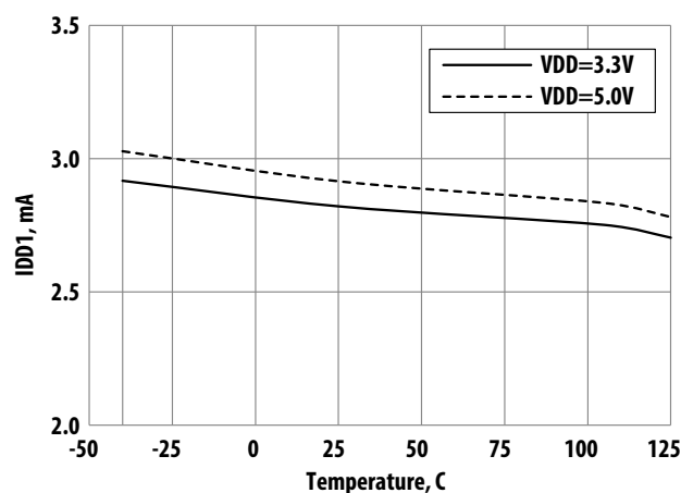
Figure 1 Typical I_{DD1(O)} vs Temperature
