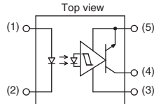
Internal circuit
