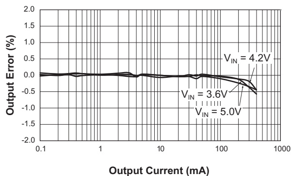
DC Regulation ( V_{OUT} = 3.3V )
