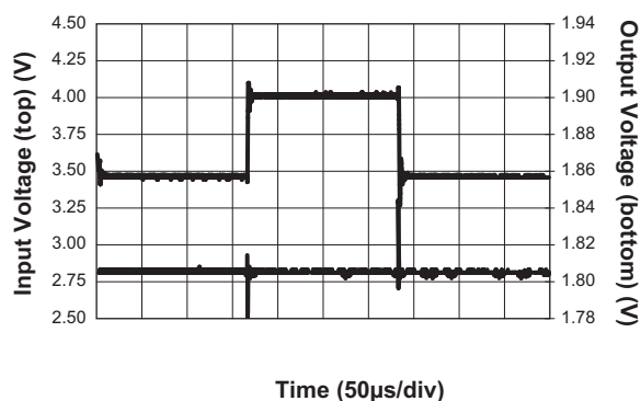
Line Transient
