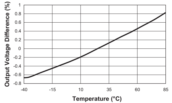
V_{OUT} Tolerance vs. Temperature ( V_{OUT} = 3.3\text{V} ; I_{LOAD} = 3\text{A} )
