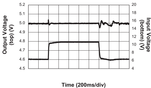
Line Transient
