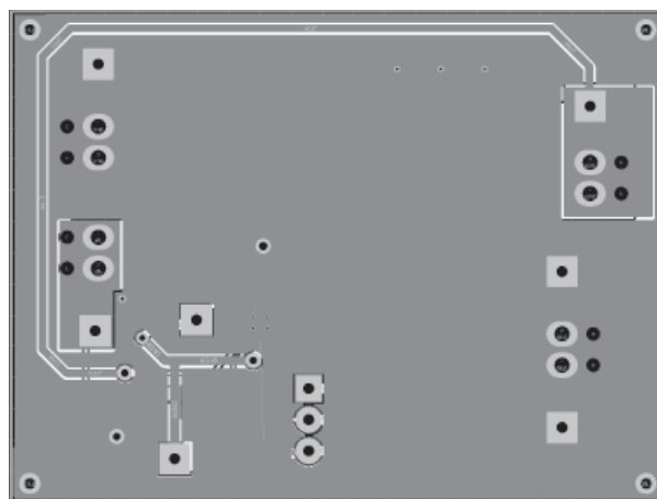
Figure 4: AAT1161 Evaluation Board Bottom Side Layout.
