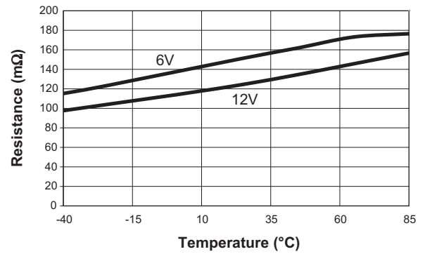
P-Channel R_{DS(ON)} vs. Temperature ( V_{IN} = 6\text{V} )
