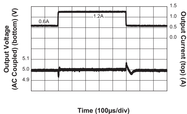
Step-Down Converter Load Transient Response ( I_{OUT} = 0.6A to 1.2A ; V_{IN} = 12V ; V_{OUT} = 5V ; C_{OUT} = 2 \times 22\mu F )
