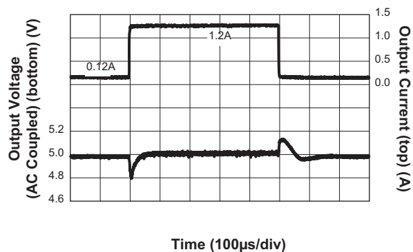
Step-Down Converter Load Transient Response ( I_{OUT} = 0.12A to 1.2A ; V_{IN} = 12V ; V_{OUT} = 5V ; C_{OUT} = 2x22μF )
