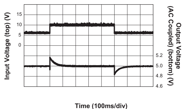
Step-Down Converter Line Transient Response ( V_{IN} = 6V to 10V ; V_{OUT} = 5V ; I_{OUT} = 1.2A )
