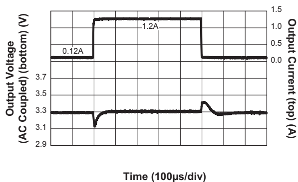
Step-Down Converter Load Transient Response ( I_{OUT} = 0.12A to 1.2A ; V_{IN} = 12V ; V_{OUT} = 3.3V ; C_{OUT} = 2x22μF )
