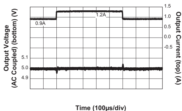
Step-Down Converter Load Transient Response ( I_{OUT} = 0.9A to 1.2A ; V_{IN} = 12V ; V_{OUT} = 5V ; C_{OUT} = 2 \times 22\mu F )
