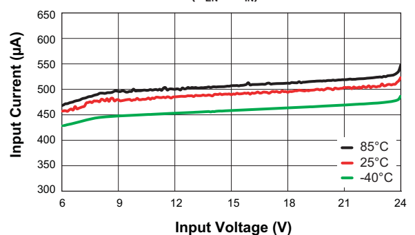
No Load Step-Down Converter Input Current vs. Input Voltage (V_{EN} = V_{IN})
