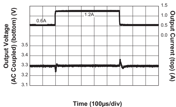
Step-Down Converter Load Transient Response ( I_{OUT} = 0.6A to 1.2A ; V_{IN} = 12V ; V_{OUT} = 3.3V ; C_{OUT} = 2 \times 22\mu F )
