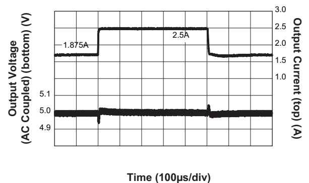
Step-Down Converter Load Transient Response ( I_{OUT} = 1.875A to 2.5A ; V_{IN} = 12V ; V_{OUT} = 5V ; C_{OUT} = 2x22\mu F )
