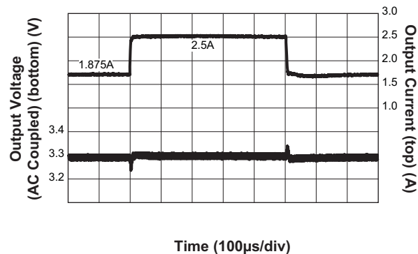
Step-Down Converter Load Transient Response ( I_{OUT} = 1.875A to 2.5A ; V_{IN} = 12V ; V_{OUT} = 3.3V ; C_{OUT} = 2x22\mu F )
