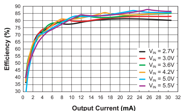
Efficiency vs. Output Current ( R_{SET} = 10k\Omega , L = 10\mu H , 6 LEDs)
