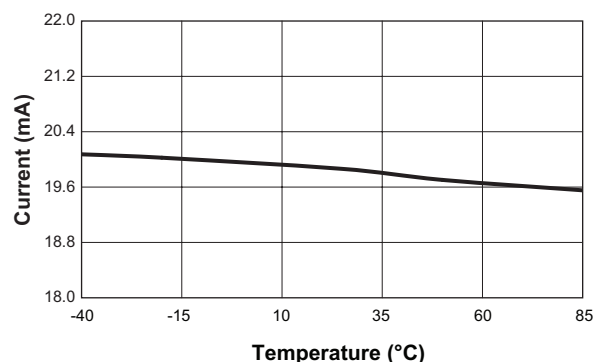
Sink Current Accuracy vs. Temperature ( V_{IN} = 3.6V , R_{SET} = 15k\Omega )
