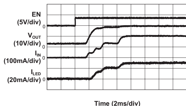
Startup Waveform
