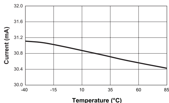
Sink Current Accuracy vs. Temperature ( V_{IN} = 3.6V , R_{SET} = 10k\Omega )
