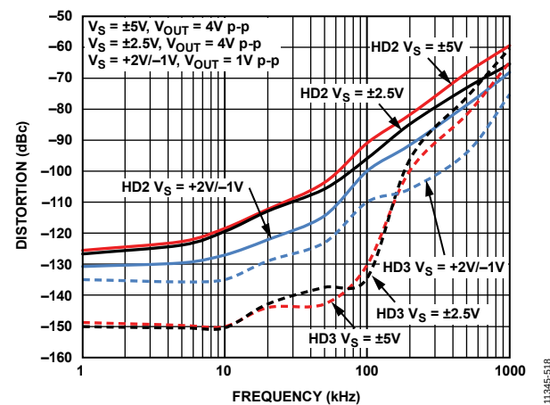
Figure 19. Distortion vs. Frequency, G = +2
