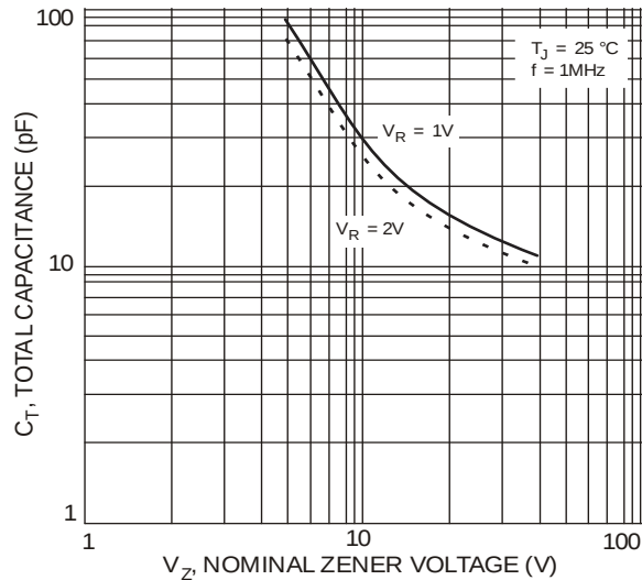
Fig. 6 Typical Total Capacitance vs. Nominal Zener Voltage
