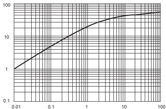
FIG. 5-TYPICAL TRANSIENT THERMAL IMPEDANCE
