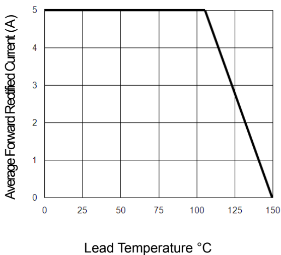
Fig.1-Forward Derating Curve
