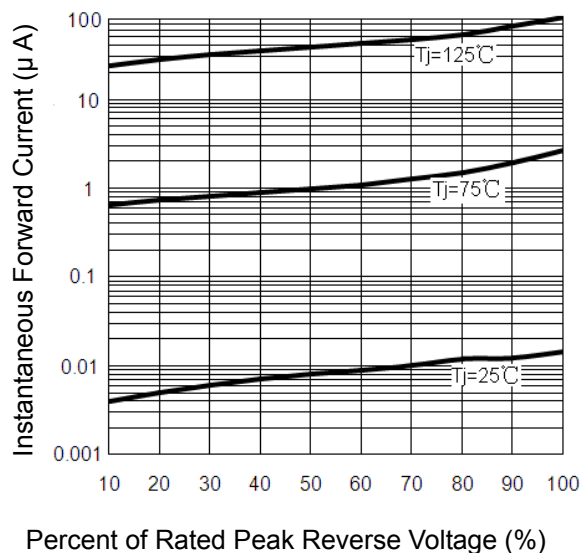
Fig.4-Typical Reverse Characteristic
