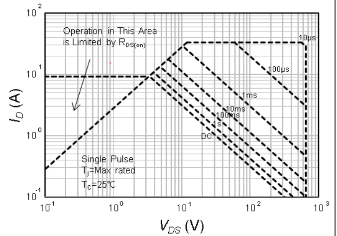
Fig.14 Maximum Safe Operating Area
