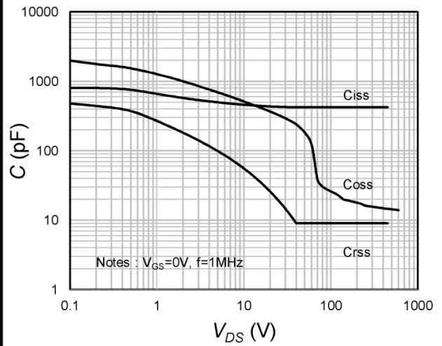
Fig.8 Capacitance Characteristics
