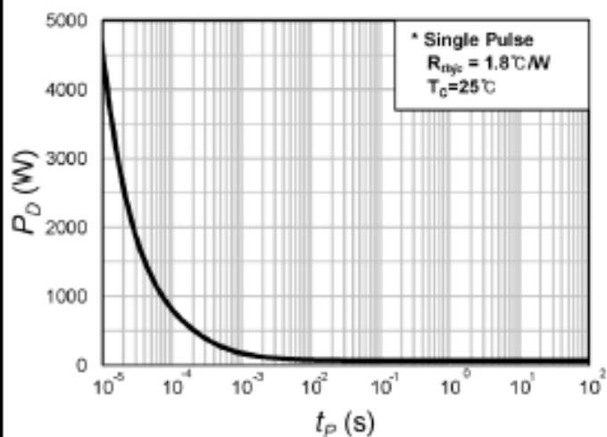
Fig.11 Single Pulse Maximum Power Dissipation
