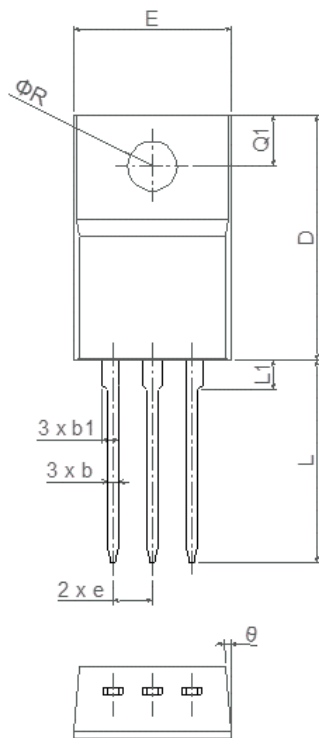
TO-220FT(For ASE ) PACKAGE OUTLINE DRAWING
