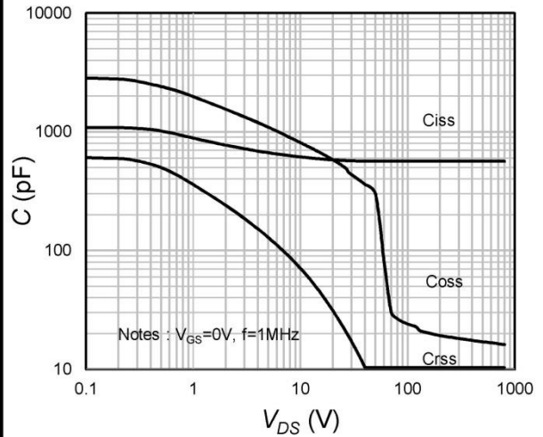
Fig.8 Capacitance Characteristics
