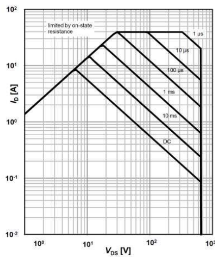
Figure 12: Maximum Forward Biased Safe Operating Area, T c =25°C TO-220FullPAK
