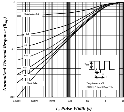
Fig 10. Effective Transient Thermal Impedanc
