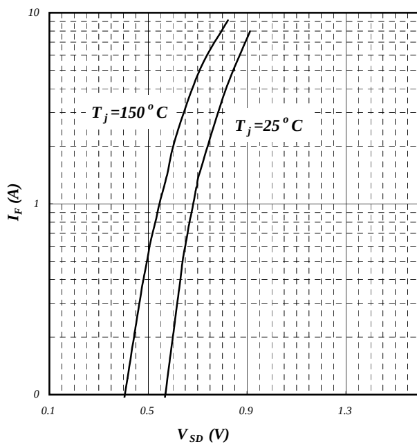
Fig 11. Forward Characteristic of Reverse Diode
