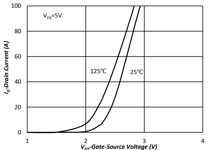
Fig.6 Transfer Characteristics
