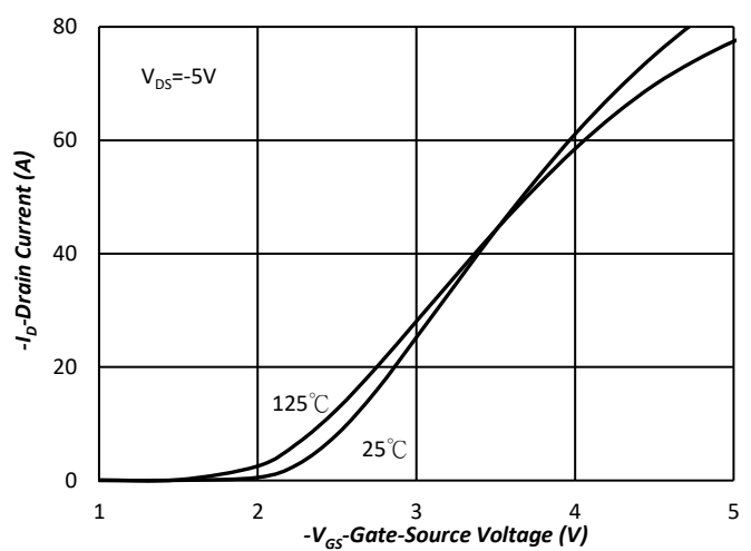
Fig.6 Transfer Characteristics
