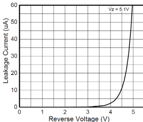
Leakage current vs. Reverse voltage
