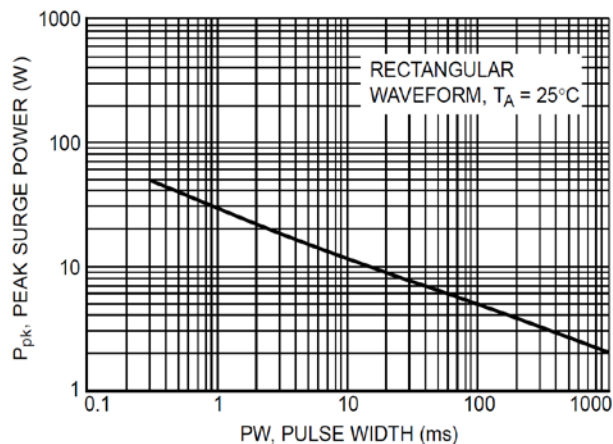
Peak surge power vs. Pulse width
