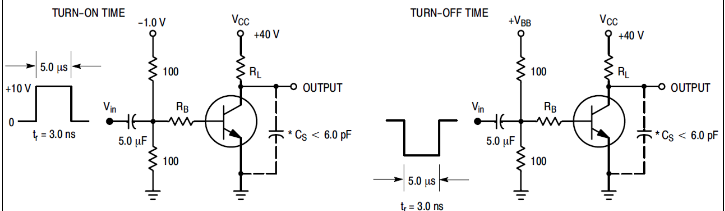
FIG.1 - Switching time test circuits
