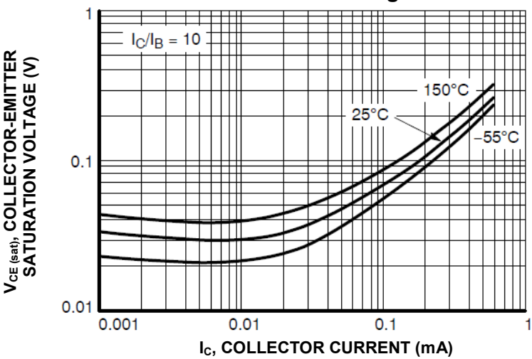
FIG.6 - Collector emitter saturation voltage vs. collector current
