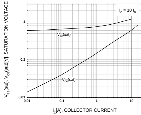
Figure 2. Base-Emmitter Saturation Voltage Collector-Emmitter Saturation Voltage
