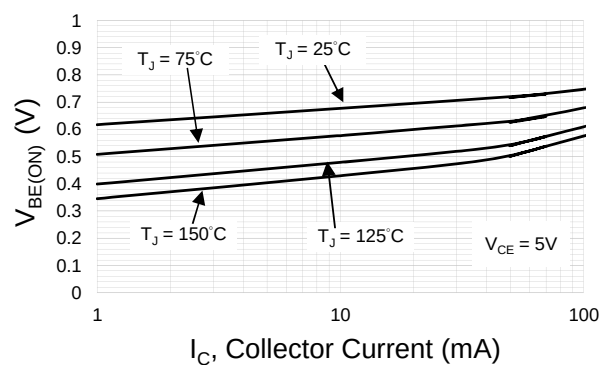
Fig.4 Typical Base - Emitter Voltage vs Collector Current
