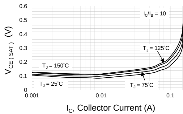
Fig.2 Typical Collector-Emitter Saturation Voltage
