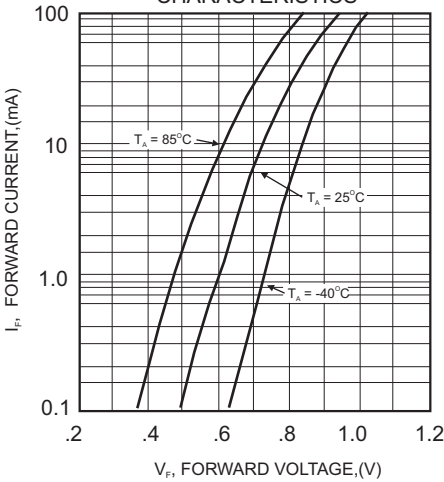
FIG.1-TYPICAL FORWARD CHARACTERISTICS
