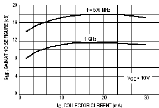
Figure 4. Gain at Noise Figure versus Collector Current
