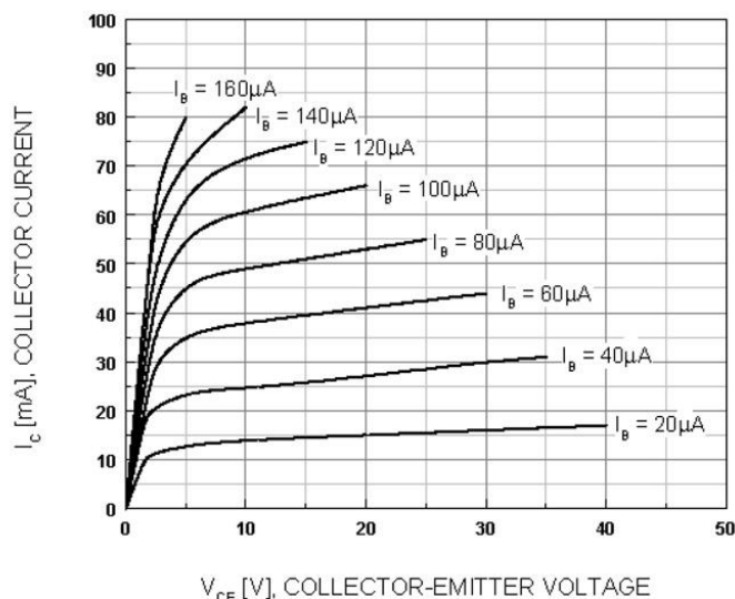
Figure 1. Static Characteristic
