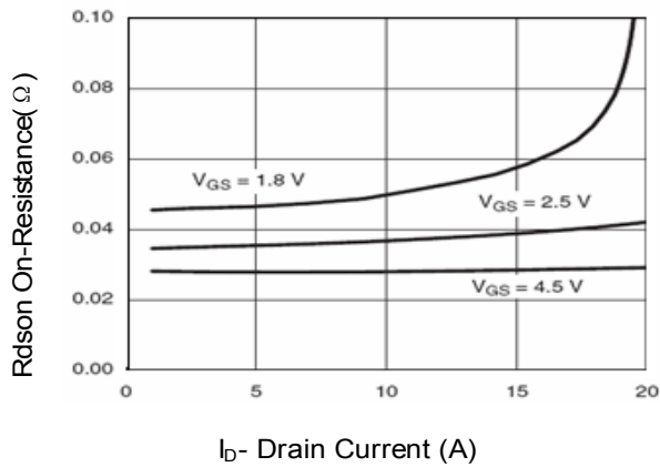
Figure 3: Drain-Source On-Resistance
