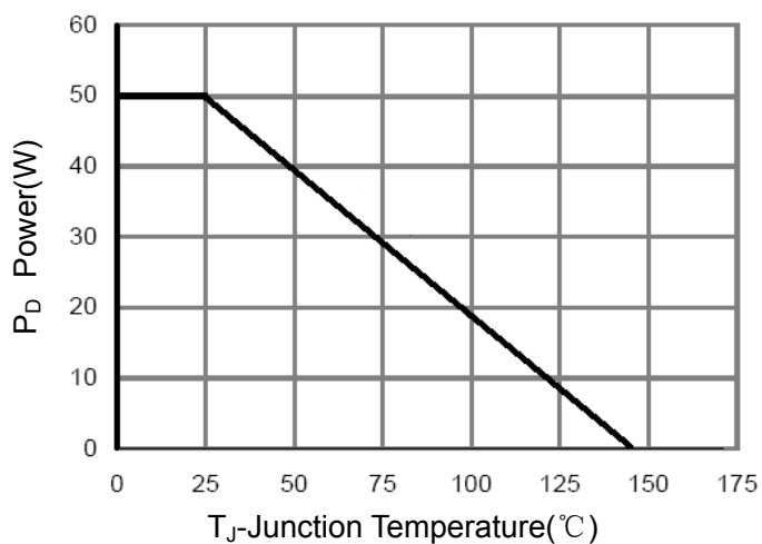
Figure 3 Power Dissipation
