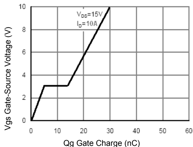
Figure 11 Gate Charge
