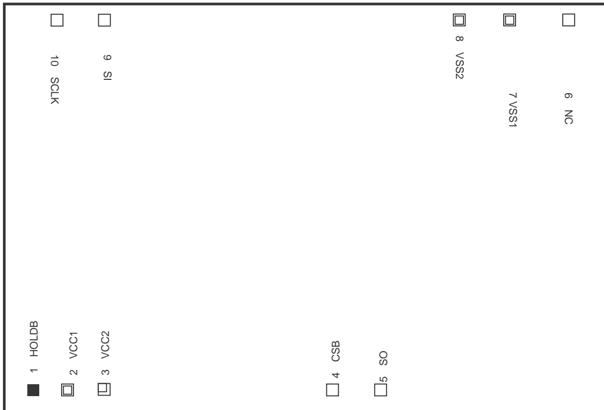
FIGURE 1. DIE PAD LOCATIONS
