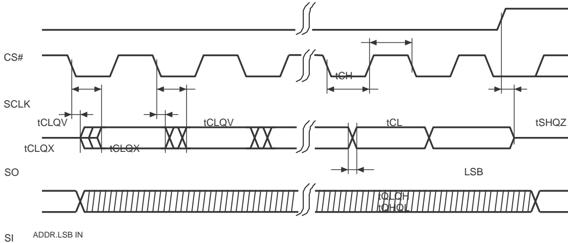
Figure 11. Output Timing
