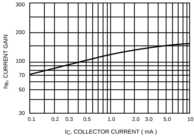
Figure 11. Current Gain
