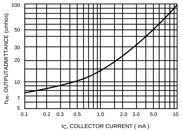
Figure 10. Output Admittance
