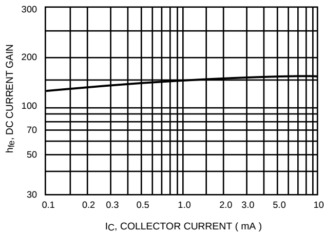
Figure 9. Current Gain
