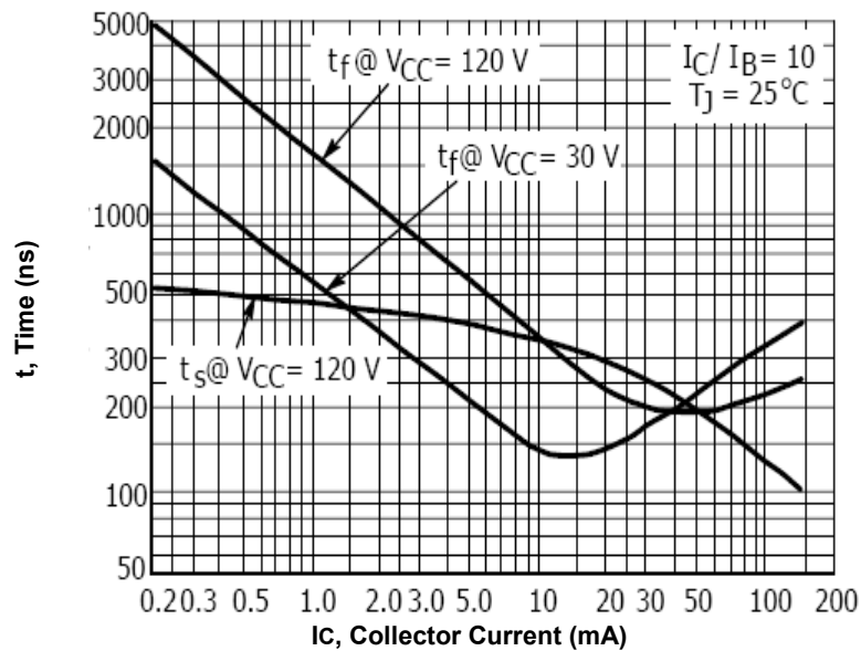
Fig.9- Turn-Off Time
