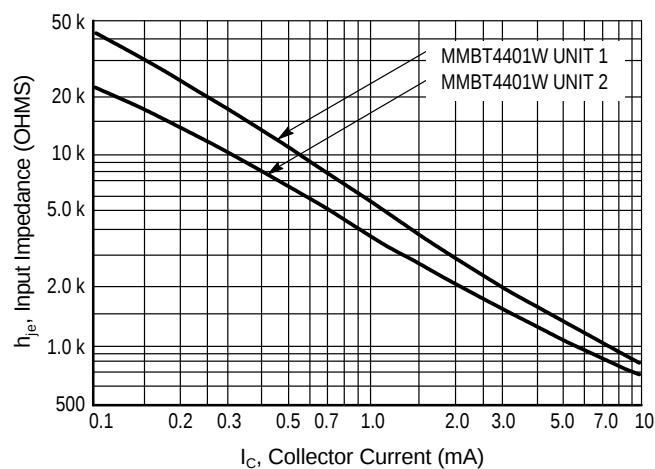
Figure 12. Input Impedance
