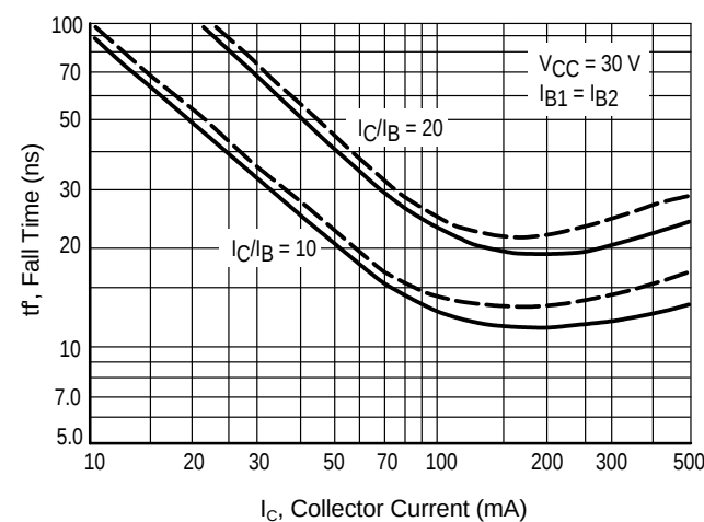
Figure 8. Fall Time
