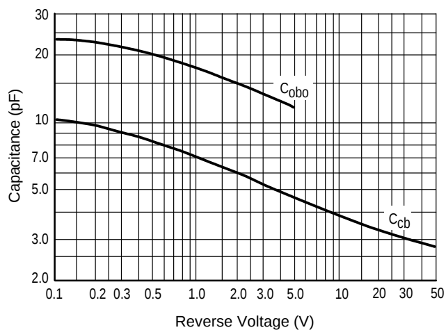
Figure 3. Capacitances
