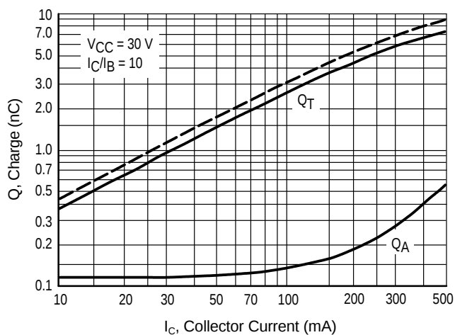
Figure 4. Charge Data
