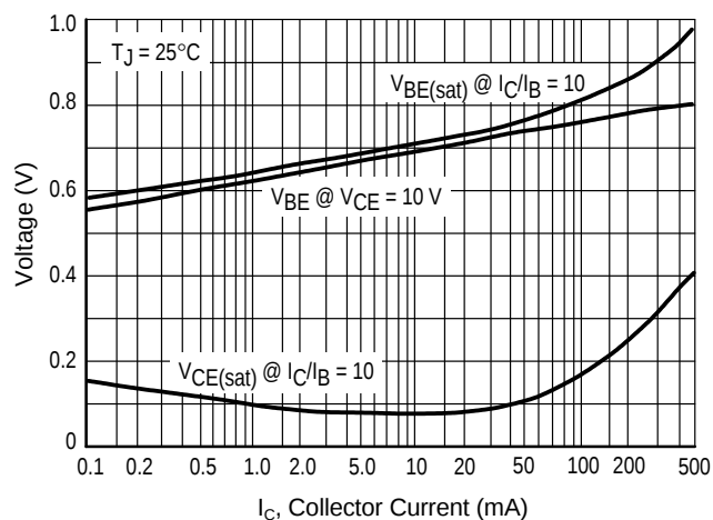
Figure 17. "On" Voltages
