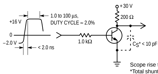
Figure 1. Turn–On Time
