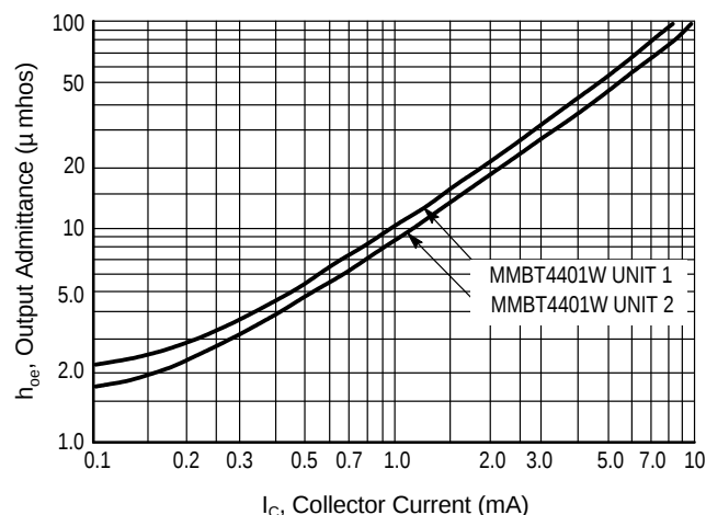
Figure 14. Output Admittance
