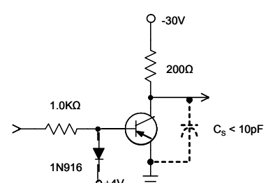
Fig. 2. Turn-Off Time
