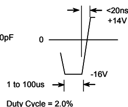
Fig. 2. Turn-Off Time
