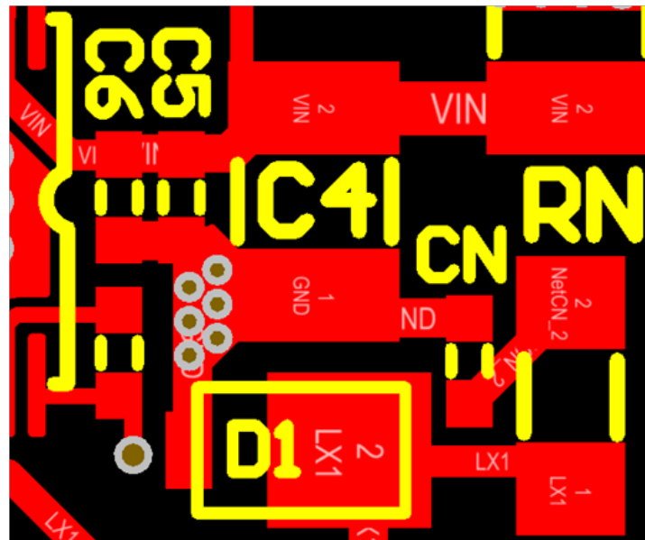
Figure 19: PCB Layout #2
