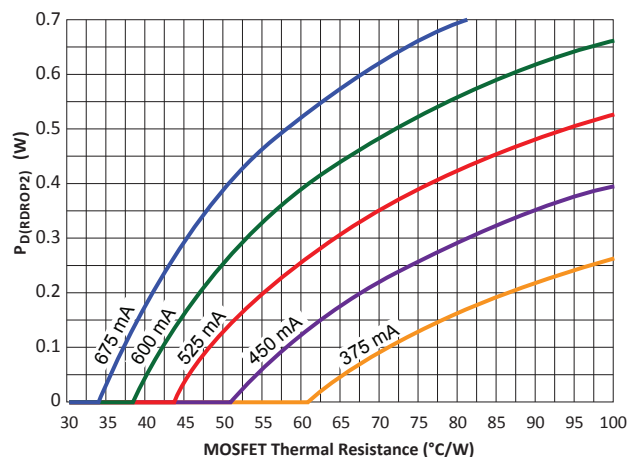
Figure 15. R_{DRO2} power dissipation versus 1.5 V MOSFET thermal resistance at various 1.5 V regulator maximum current settings
