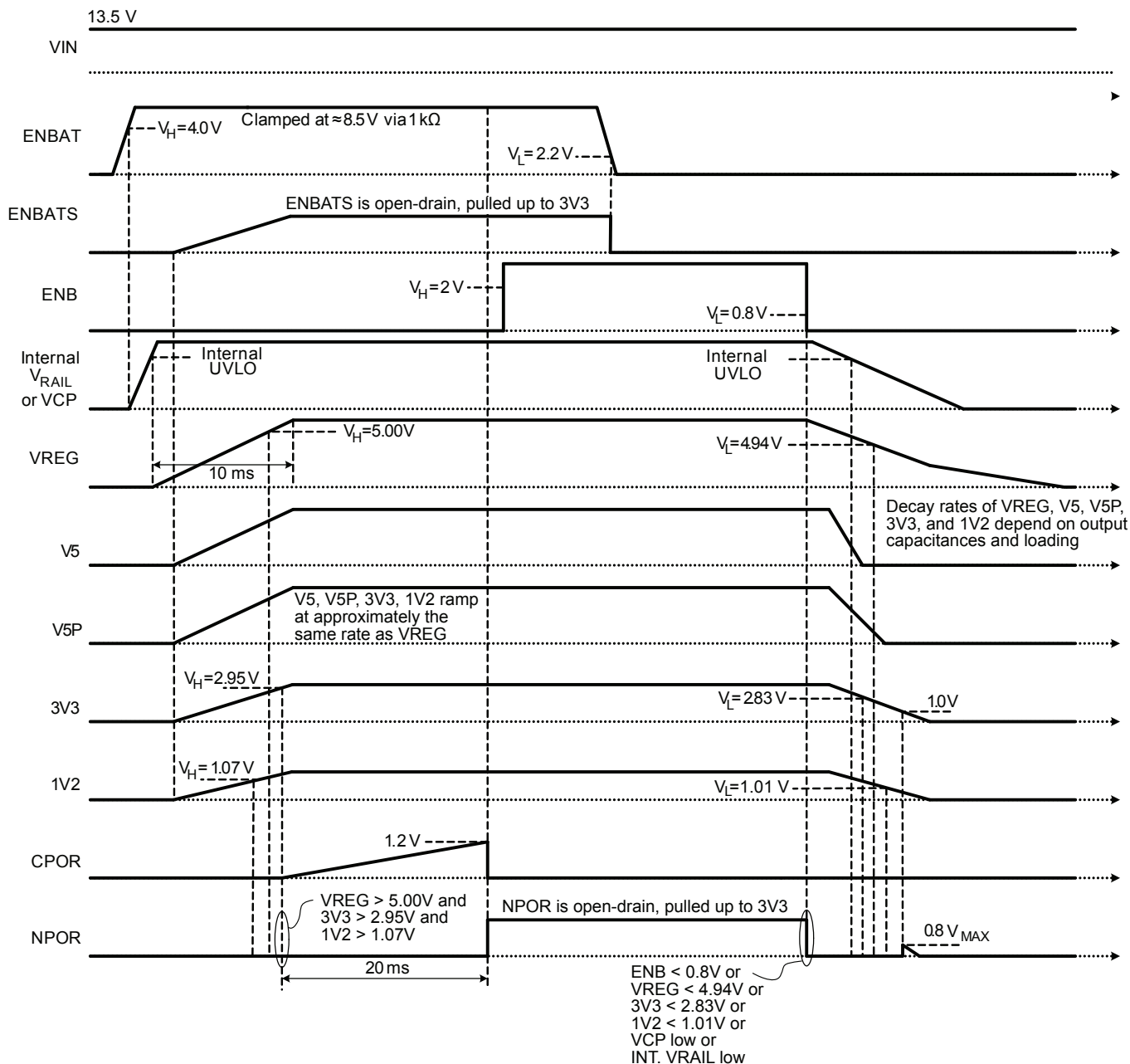
Figure 10. Typical power-up and power-down by ENBAT and ENB with V_{IN} = 13.5\text{ V} ; ENBATS is assumed to be connected to 3V3 via a pull up resistor
