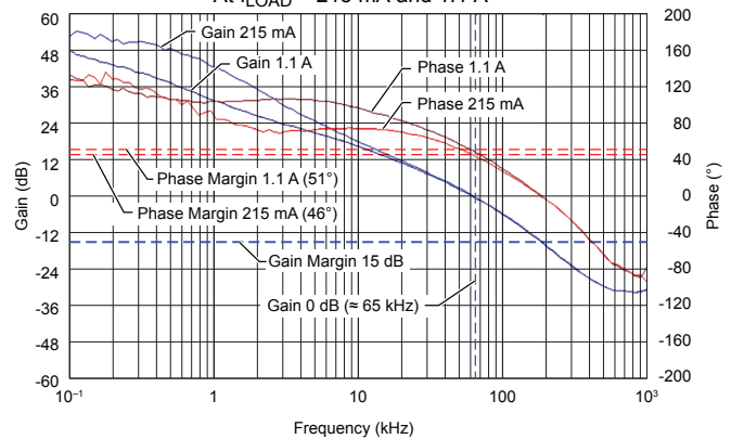
Buck Regulator Bode Plots
