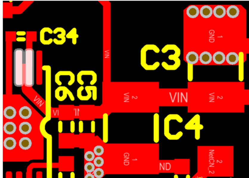
Figure 23: PCB Layout #1
