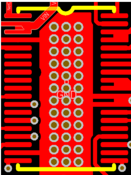
Figure 33: PCB Layout #11
