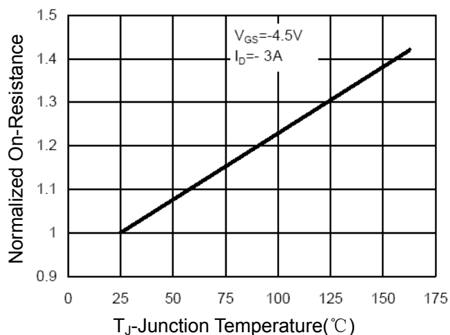
Figure 8 Drain-Source On-Resistance
